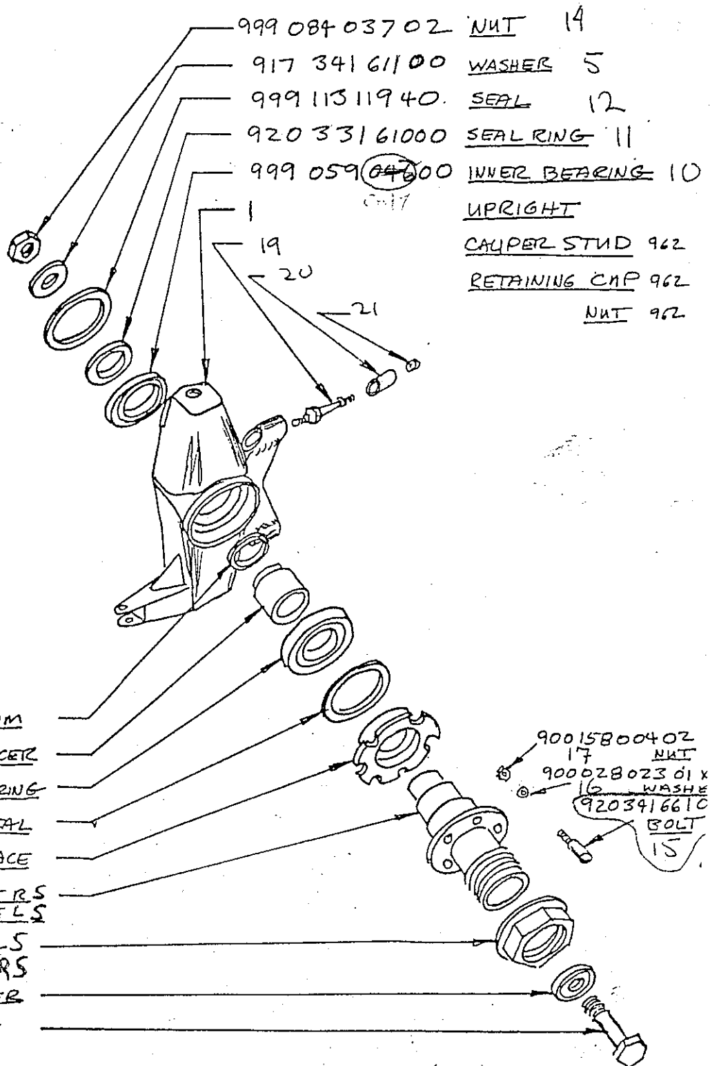
944 GTR FRONT UPRIGHT LEFT SIDE SHOWN
