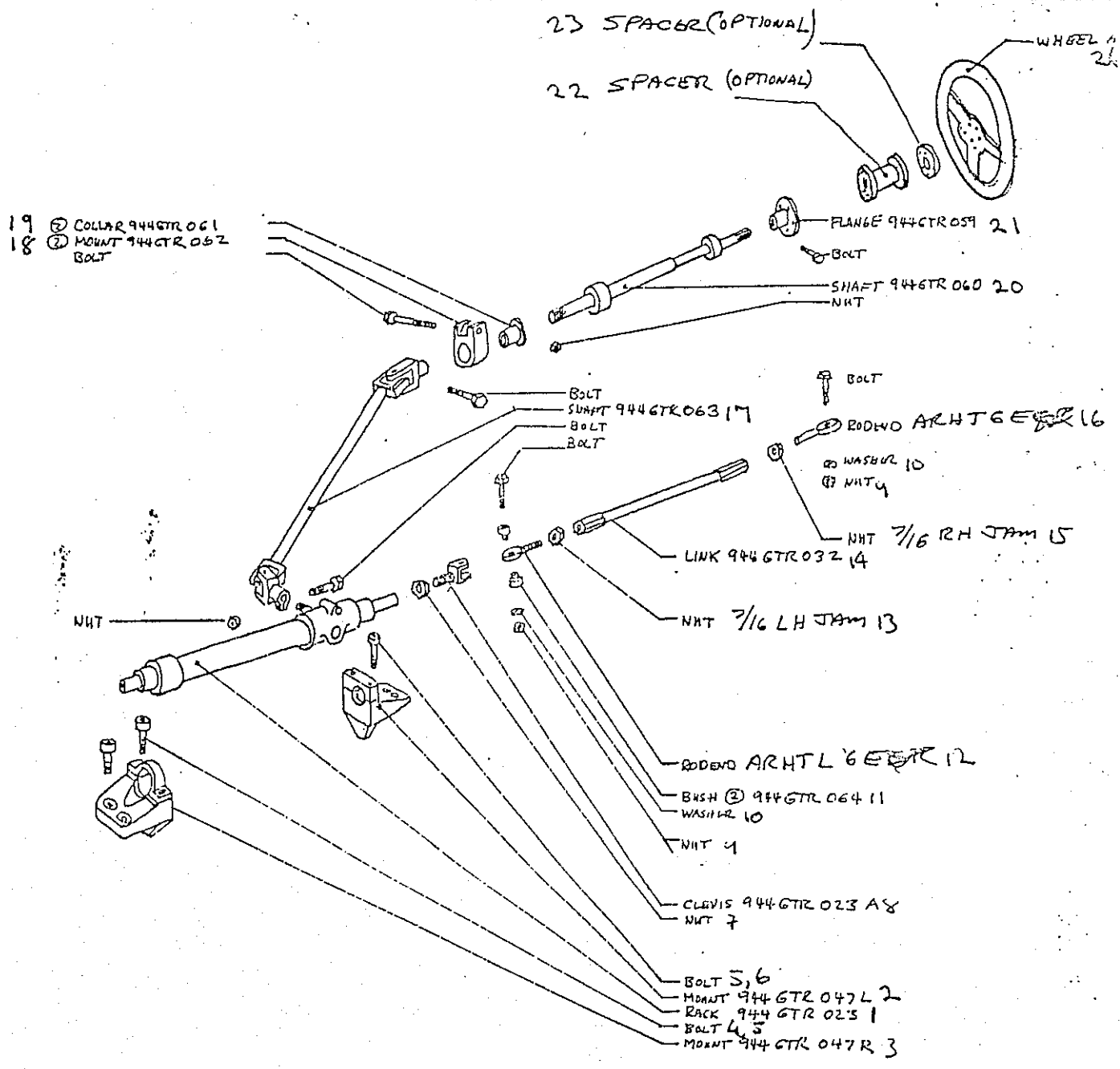
944 STEERING COMPONENTS JULY 1985
